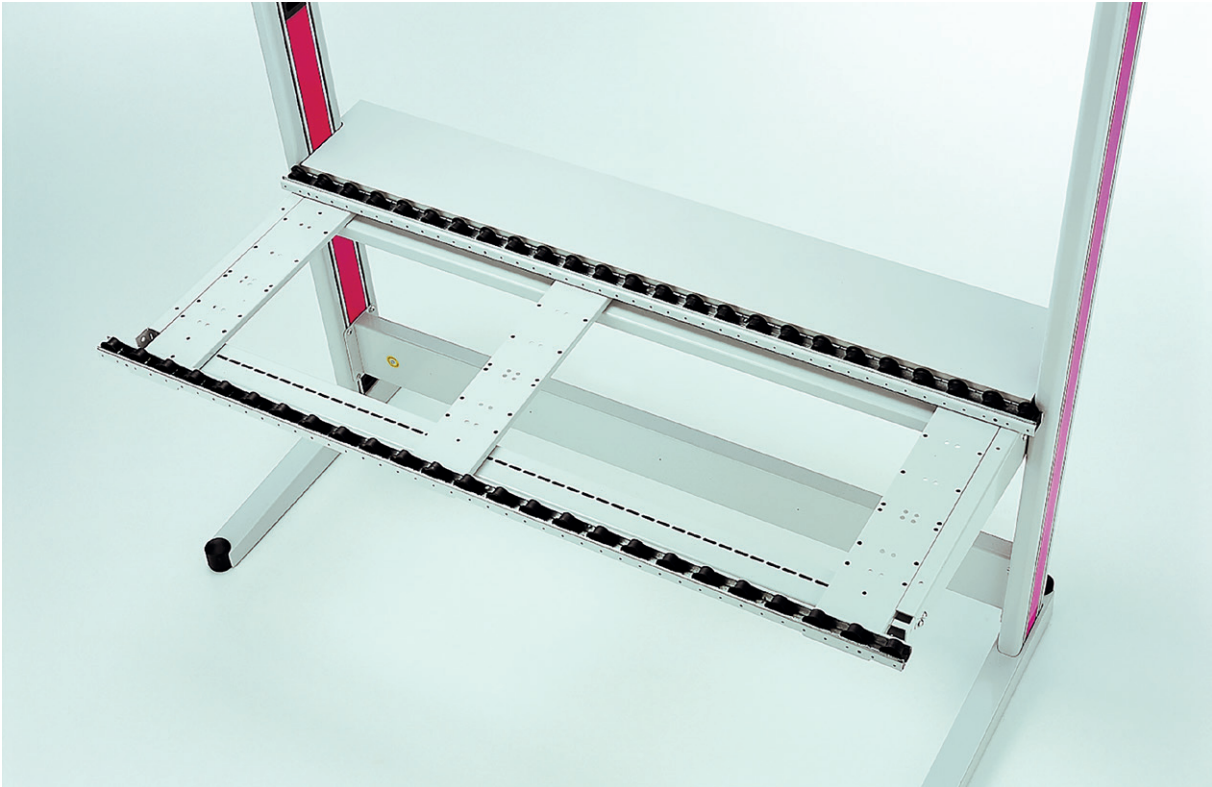
Roller tracks across the entire table width
